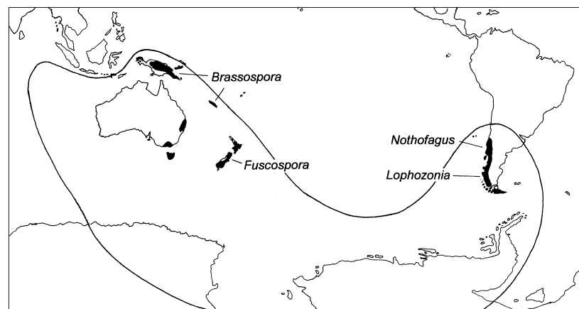
Figure 1 Distribution of Nothofagus : fossils (continuous line, including the Ninety East Ridge and Antarctica), extant distribution (solid black), and main massings (extant and fossil plus extant) of the four extant subgenera.
